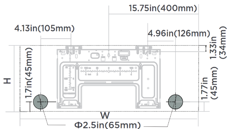
Indoor unit dimensions(WxH): 28.7in(729mm)x11.5in(293mm)
